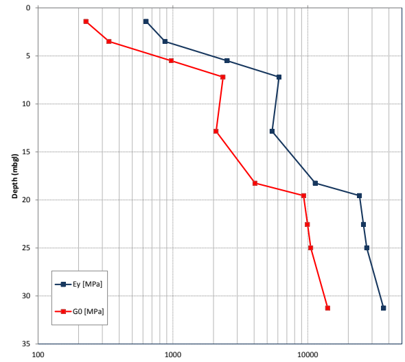
Geotechnical foundation design parameters
