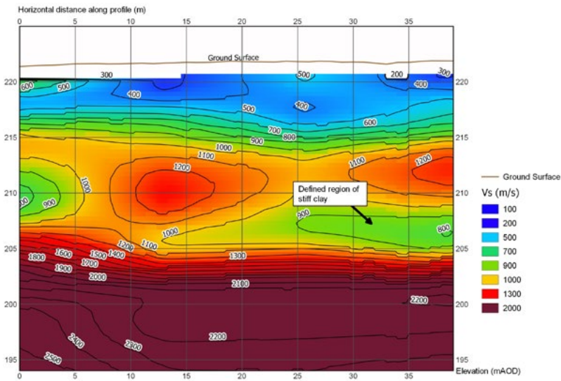
2D S-Wave velocity profile
