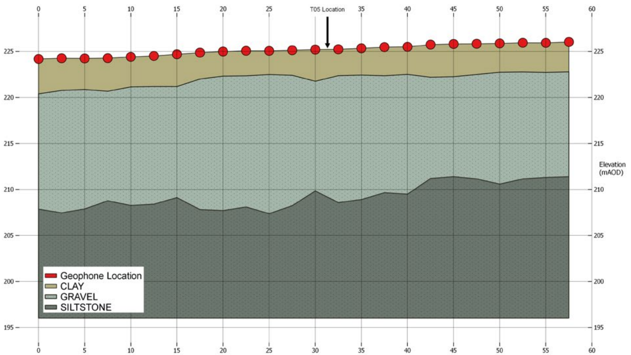
Seismic refraction ground profile (A-B)
