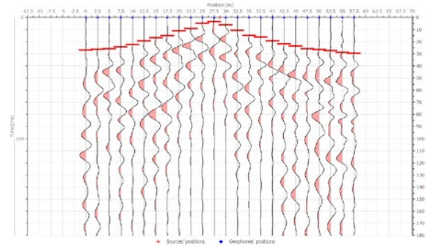
2D seismic wave traces recorded by the seismometer on site
